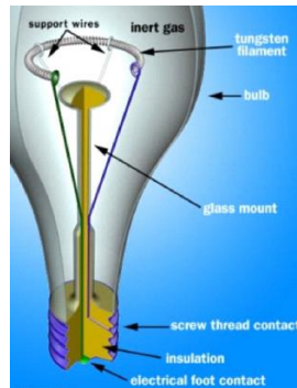
Figure 3 Details of incandescent lamp [3]
